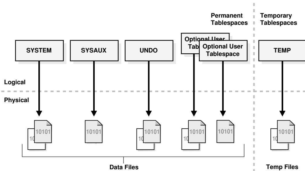
Figure 12-28 Tablespaces
