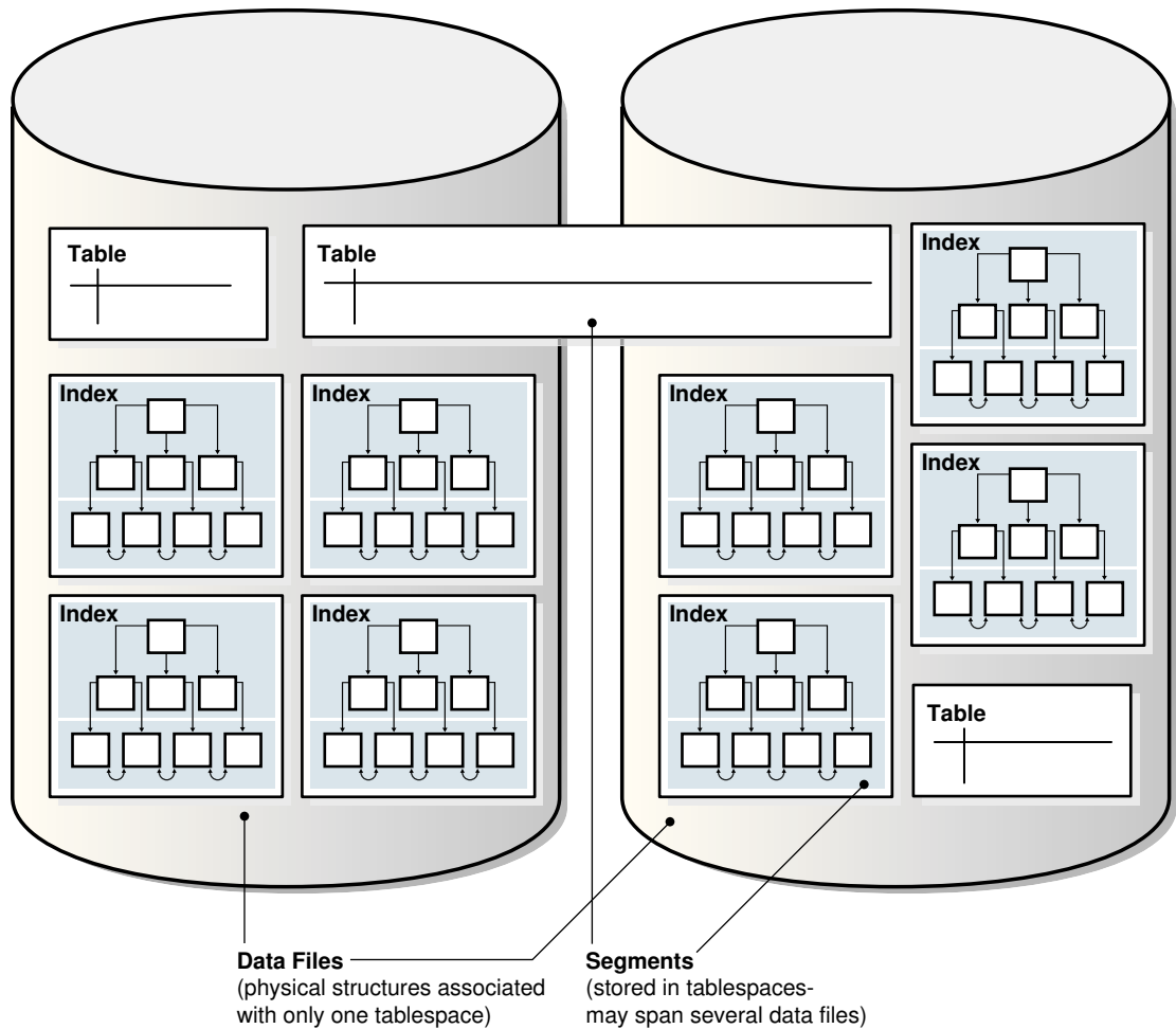
Figure 7-2 Optimizer Components
