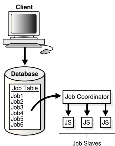
Figure 18-8 Scheduler Components
