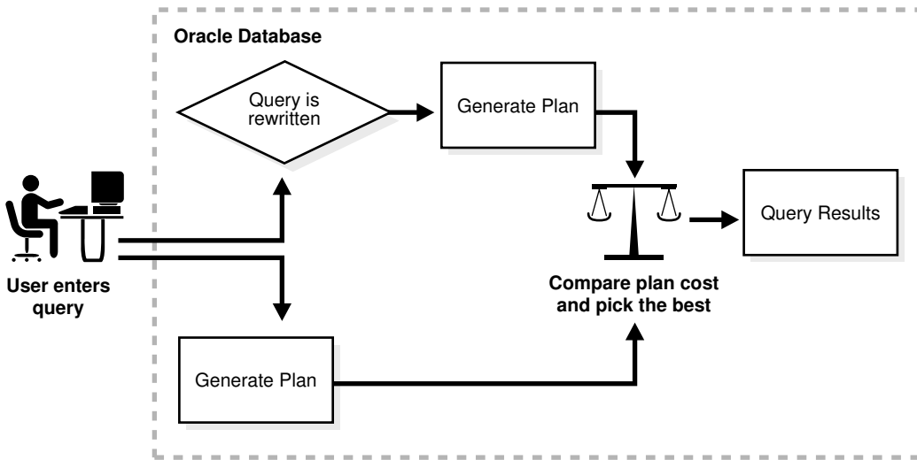
Figure 4-10 Query Rewrite
