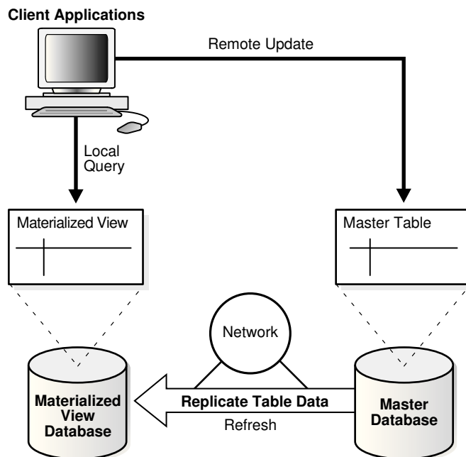
Figure 4-9 Materialized View
